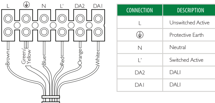
Figure 8: Wiring schematic
