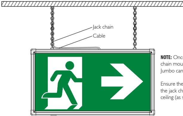
Figure 7: Jack chain installation
